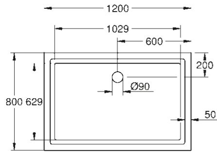
39 305 000* Universal shower tray 80 cm x 120 cm
