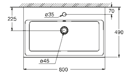
39 469 00H Wall hung basin 80 cm
