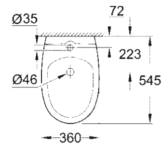
39 432 000 Floorstanding bidet
