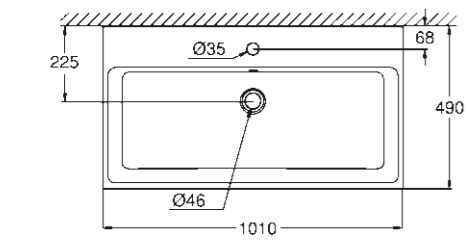
39 386 00H Wall hung basin 100 cm
